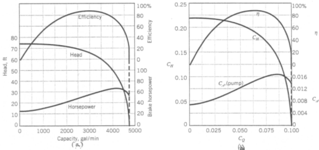
Fig 4: Performance Data for a 12-in. centrifugal Pump operating at 1000 rpm
