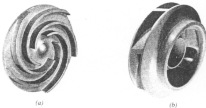
Fig 2: Open and Enclosed Impeller
