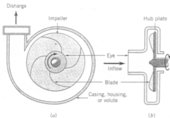
Fig 1: Centrifugal Pump
