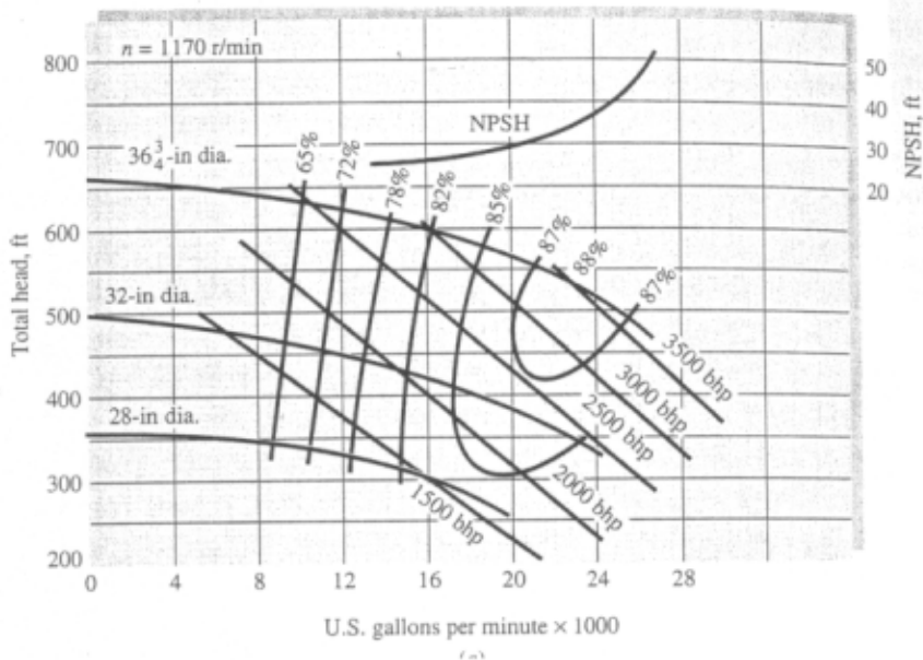
Fig 3: Performance Curve for a centrifugal Water Pump
